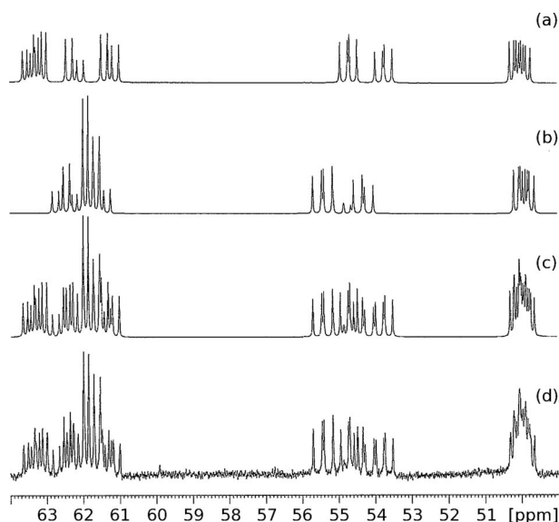
Figure 2. (a) Simulated ^{31}\text{P}\{^1\text{H}\} NMR spectrum of 2f . (b) Simulated spectrum of 2f' . (c) Combined simulated spectra. (d) Experimental spectrum [162 MHz, (\text{CD}_3)_2\text{CO} ].
