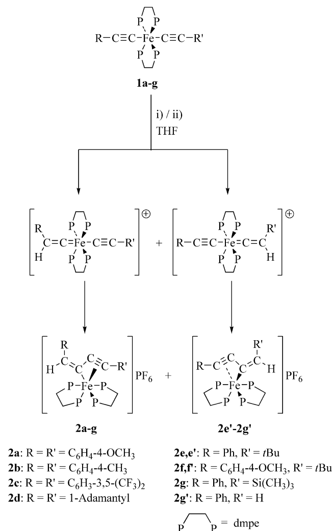
Scheme 3. Preparation of butenynyl-iron(II) complexes 2a–g . Reagents: i) CF 3 COOH, KPF 6 ( 2a–2d , 2f/f' ). ii) NH 4 PF 6 ( 2e/e' , 2g/g' ).
