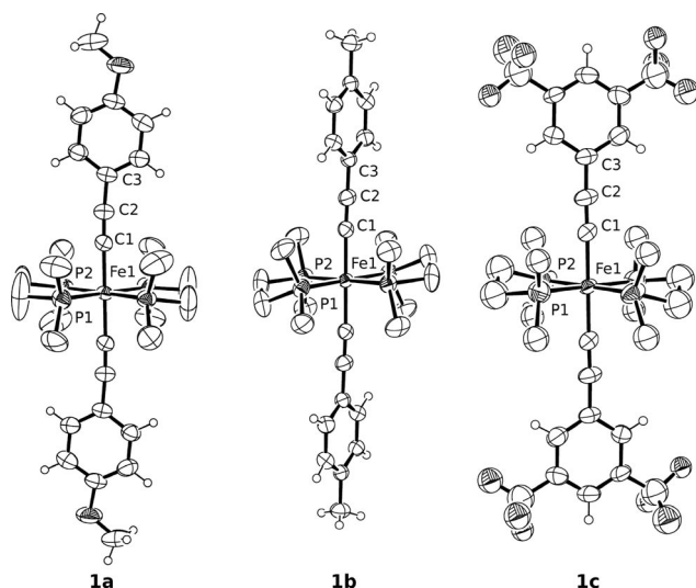
Figure 1. Molecular projection of the complexes trans -Fe(C≡C-C 6 H 4 -4-OMe) 2 (dmpe) 2 ( 1a , left), trans -Fe(C≡C-C 6 H 4 -4-Me) 2 (dmpe) 2 ( 1b , centre) and trans -Fe(C≡C-C 6 H 3 -3,5-(CF 3 ) 2 ) 2 (dmpe) 2 ( 1c , right). Thermal ellipsoids are shown at the 50% probability levels, selected hydrogen atoms have been removed for clarity.
