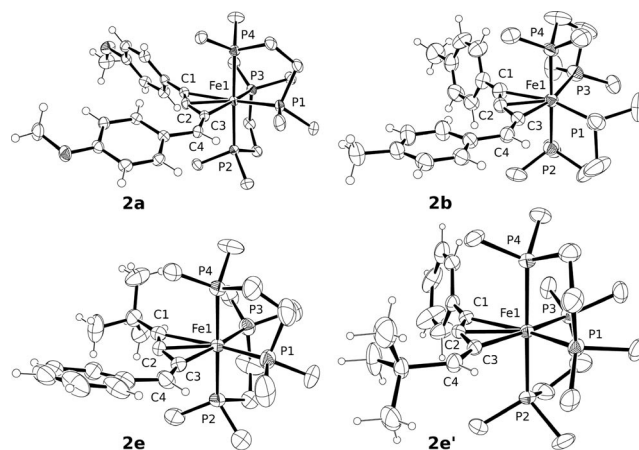
Figure 3. Molecular projection of the complex cations of 2a (top left), 2b (top right), 2e (bottom left) and 2e' (bottom right). Only one component of each of the disordered sites of 2b and 2e is shown.
